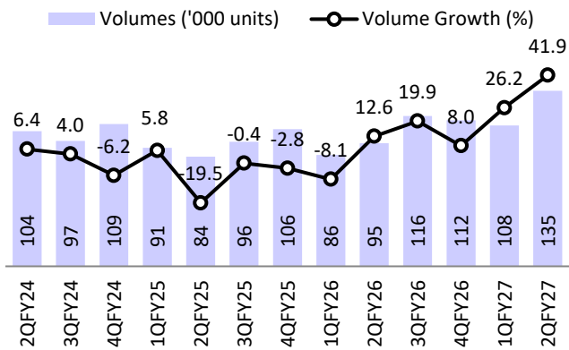
Exhibit 1: Volume trend
